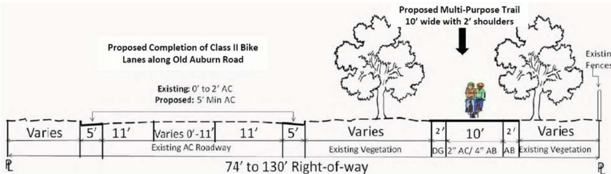
TYPICAL CROSS SECTION OF OLD AUBURN ROAD (Facing West on Old Auburn Rd.)
